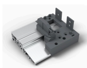
H5 Threshold connector — plastic, sill to frame · Vi6
